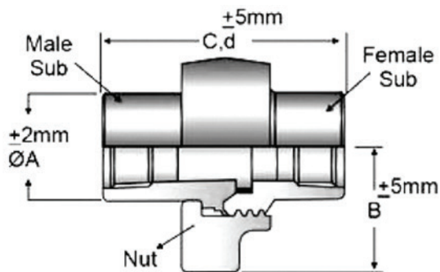
15,000 PSI CWP (FIG - 1502)
